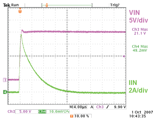
Figure 40. Adapter DC Side Hot Plug-in Test Waveforms
